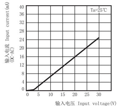
输入电压-输入电流 Input voltage-Input current
