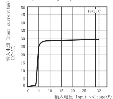
输入电压-输入电流 Input voltage-Input current
